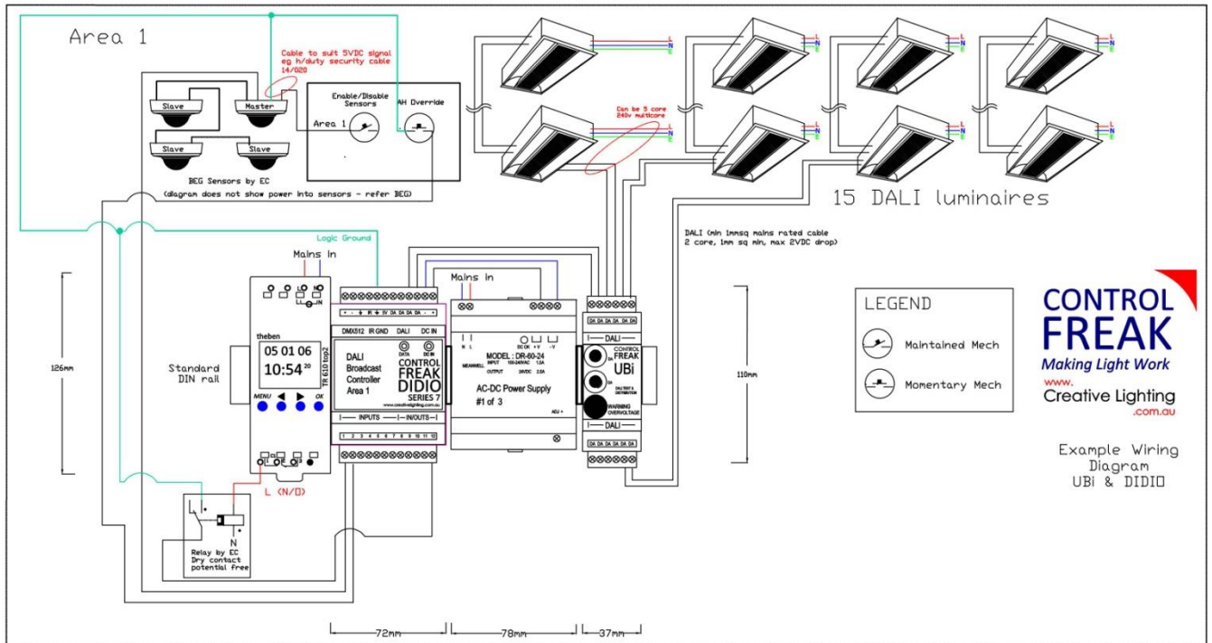
Example block wiring diagram
